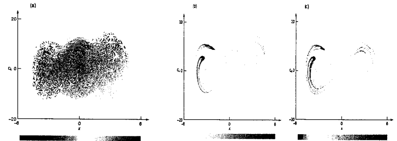
FIGURE B. Decoherence in a Chaotic Driven Double-Well System. This numerical study (Habib et al. 1998) of a chaotic driven double-well system described by the Hamiltonian H = p^2/2m - Ax^+ Bx^4 + Fx \cos(\omega t) with m = 1, A = 10, B = 0.5, F = 10 , and \omega = 6.07 illustrates the effectiveness of decoherence in the transition from quantum to classical. These parameters result in a chaotic classical system with a Lyapunov exponent \lambda \simeq 0.5 . The three snapshots taken after 8 periods of the driving force illustrate phase space distributions in (a) the quantum case, (b) the classical case, and (c) the quantum case but with decoherence ( D = 0.025 ). The initial condition was always the same Gaussian, and in the quantum cases, the state was pure. Interference fringes are clearly visible in (a), which bears only a vague resemblance to the classical distribution in (b). By contrast, (c) shows that even modest decoherence helps restore the quantum-classical correspondence. In this example the coherence length \ell_C is not much smaller than the typical nonlinearity scale, so the system is on the border between quantum and classical. Indeed, traces of quantum interference are still visible in (c) as blue “troughs,” or regions where the Wigner function is still slightly negative. The change in color from red to blue shown in the legends for (a) and (c) corresponds to a change from positive peaks to negative troughs. In the ab initio classical case (b), there are no negative troughs.
