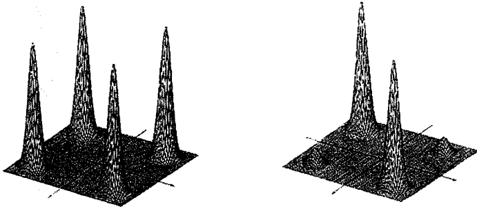
FIGURE 3. Evolution of the Density Matrix for the Schrödinger Cat State in Figure 2. (a) This plot shows the density matrix for the cat state in Figure 2 in the position representation \rho(x, x') = \varphi(x)\varphi^*(x') . The peaks near the diagonal (green) correspond to the two possible locations of the particle. The peaks away from the diagonal (red) are due to quantum coherence. Their existence and size demonstrate that the particle is not in either of the two approximate locations but in a coherent superposition of them. (b) Environment-induced decoherence causes decay of the off-diagonal terms of \rho(x, x') . Here, the density matrix in (a) has partially decohered. Further decoherence would result in a density matrix with diagonal peaks only. It can then be regarded as a classical probability distribution with an equal probability of finding the particle in either of the locations corresponding to the Gaussian wave packets.
